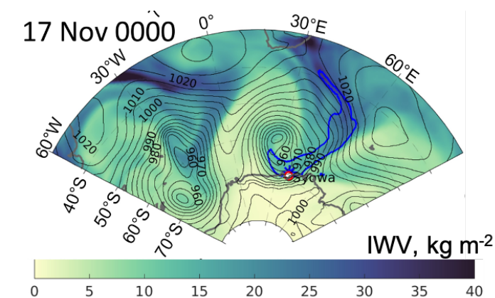
Atmospheric river affecting Syowa during YOPP on 17 November 2018 (source: Gorodetskaya et al., 2020).
