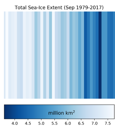
September total Arctic sea-ice extent from 1979 to 2017 (source: Thomas Rackow).
