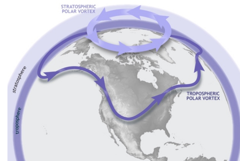
Illustration of the polar vortices in the northern hemisphere. Schematic is by NOAA Climate.gov and is adapted from Vaugh et al., 2017, Figure 1 .
