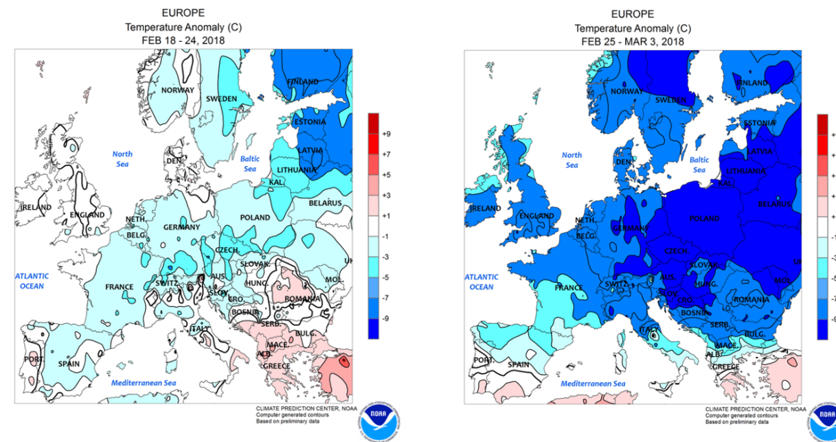
Temperature anomalies during the Beast from the East event over Europe (source: Climate Prediction Center, NOAA).
